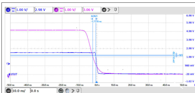
Figure 19. Turn-off Transient
