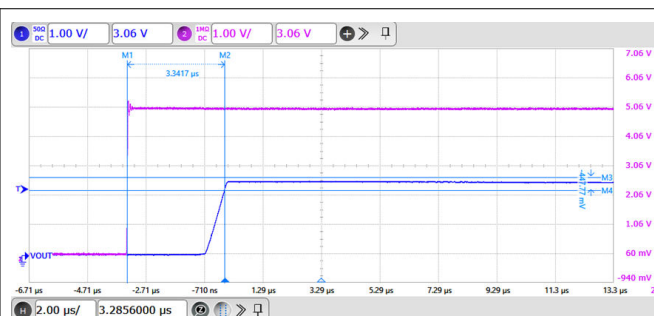
Figure 20. Turn-on Transient
